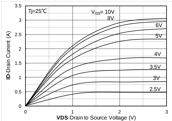
Figure 1. Output Characteristics; typical values
